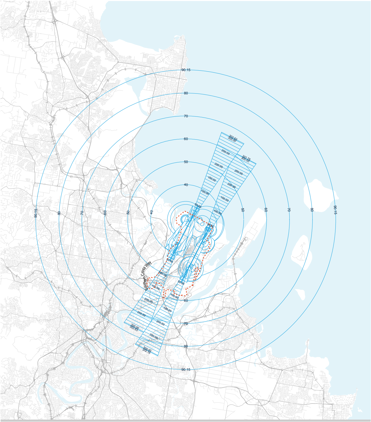
FIGURE 7.6: COMMUNICATIONS NAVIGATION AND SURVEILLANCE ASSESSMENT LEVELS
