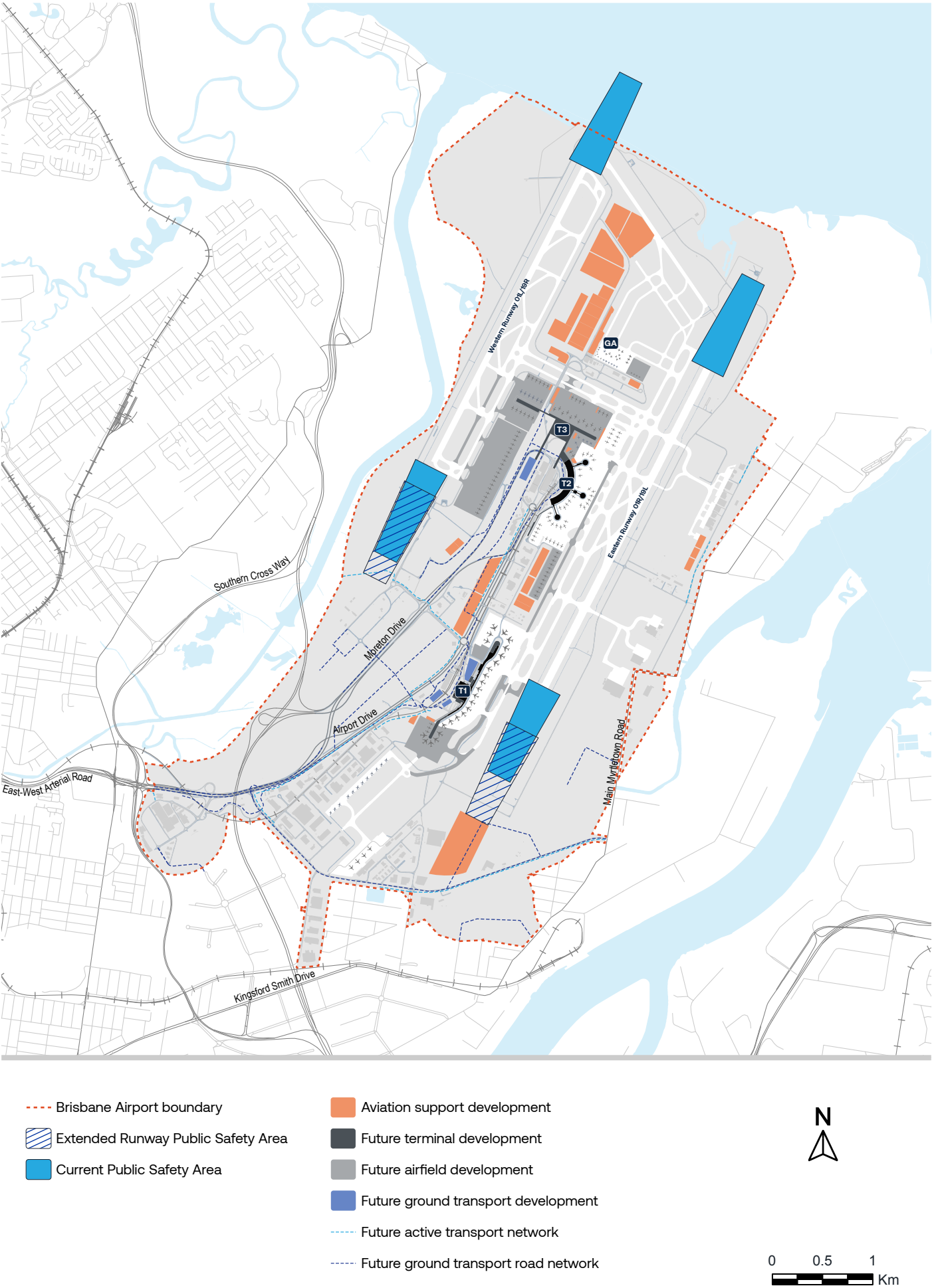
FIGURE 7.7: RUNWAY SAFETY AREAS
