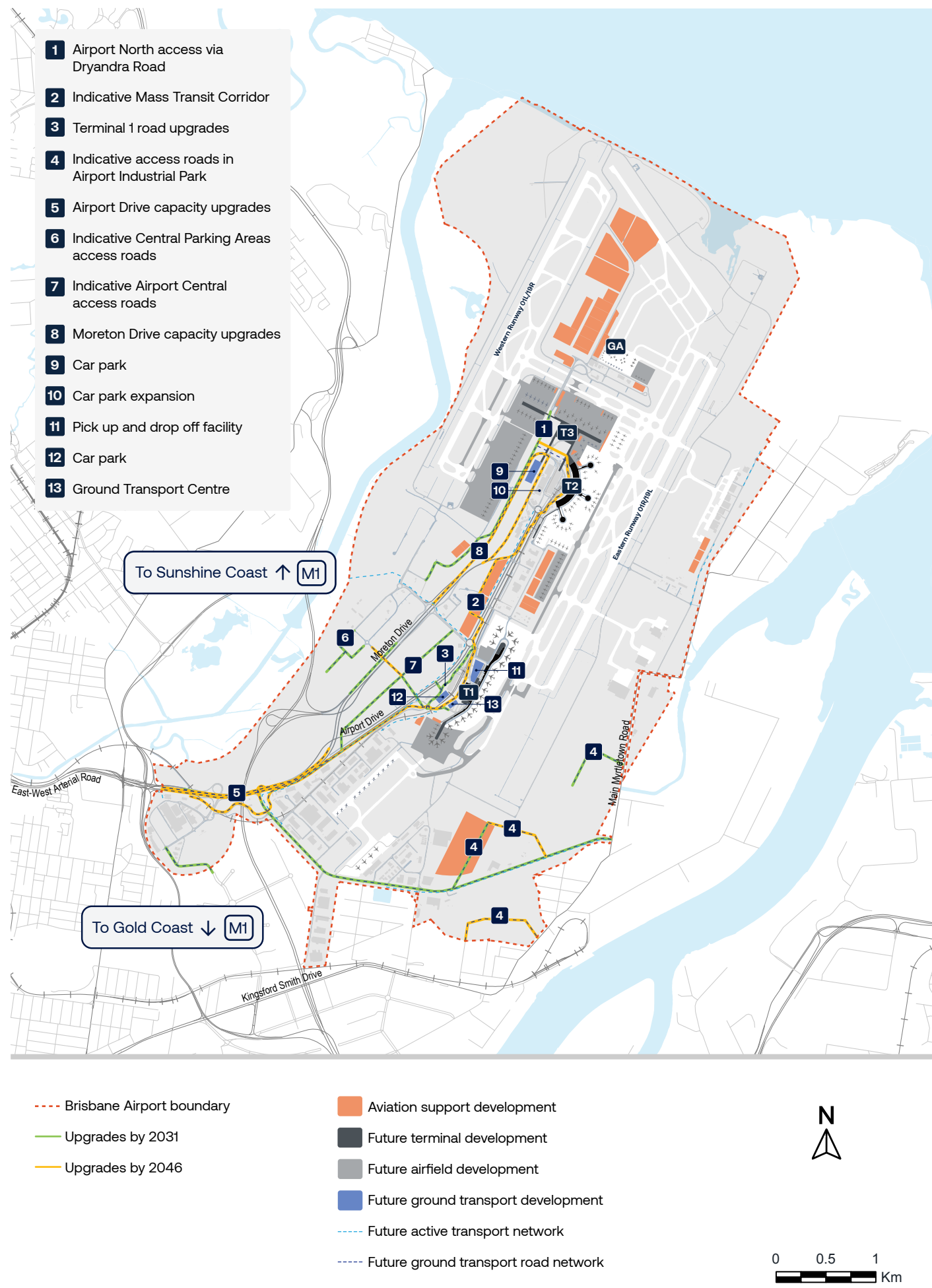
FIGURE 14.10: ON-AIRPORT FUTURE GROUND TRANSPORT DEVELOPMENT
