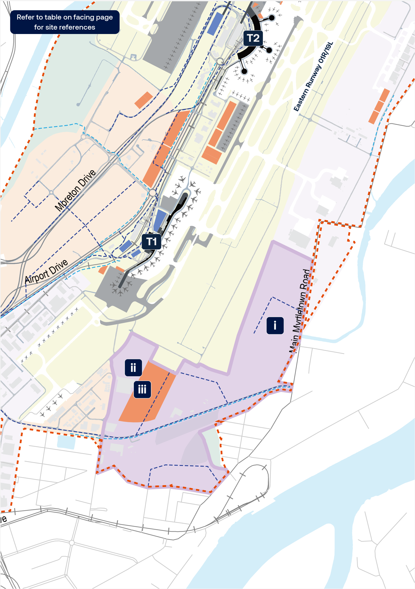
FIGURE 10.8: AIRPORT INDUSTRIAL PARK PRECINCT FIVE YEAR DEVELOPMENTS
