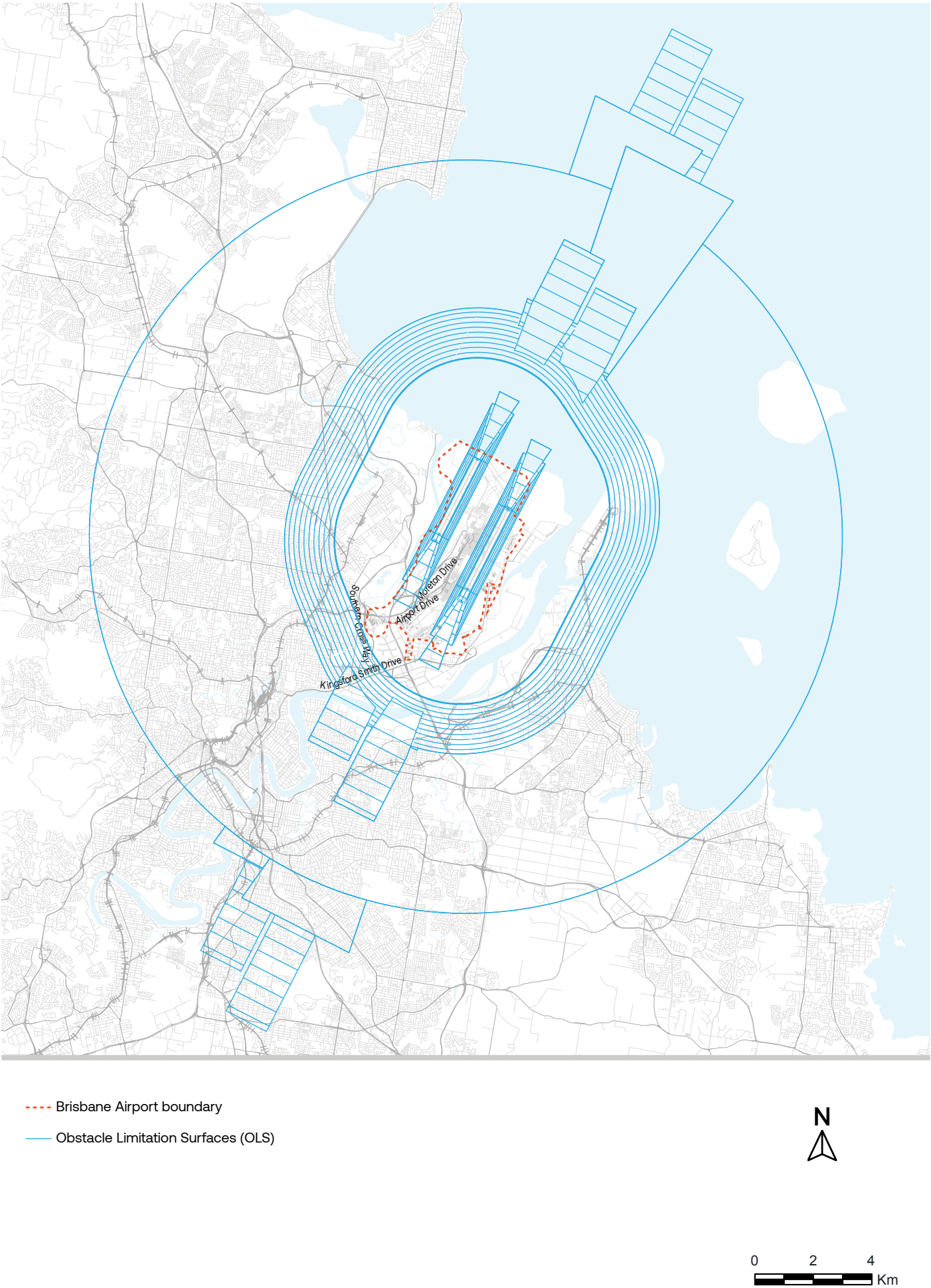
FIGURE 7.4: OBSTACLE LIMITATION SURFACE
