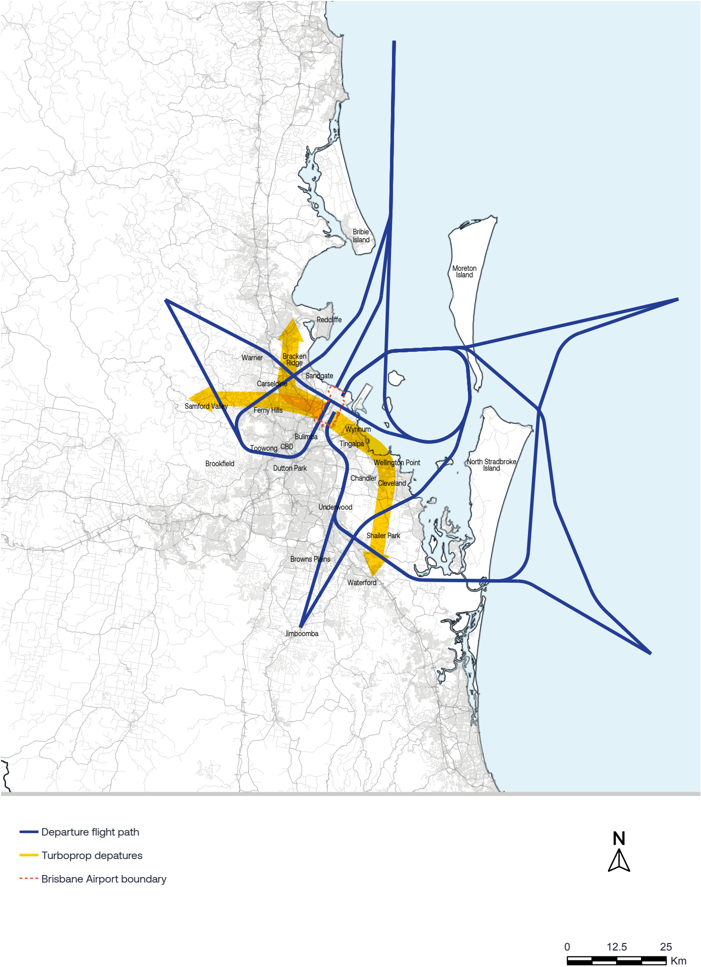
FIGURE 12.2: CURRENT DEPARTURE FLIGHT PATHS
