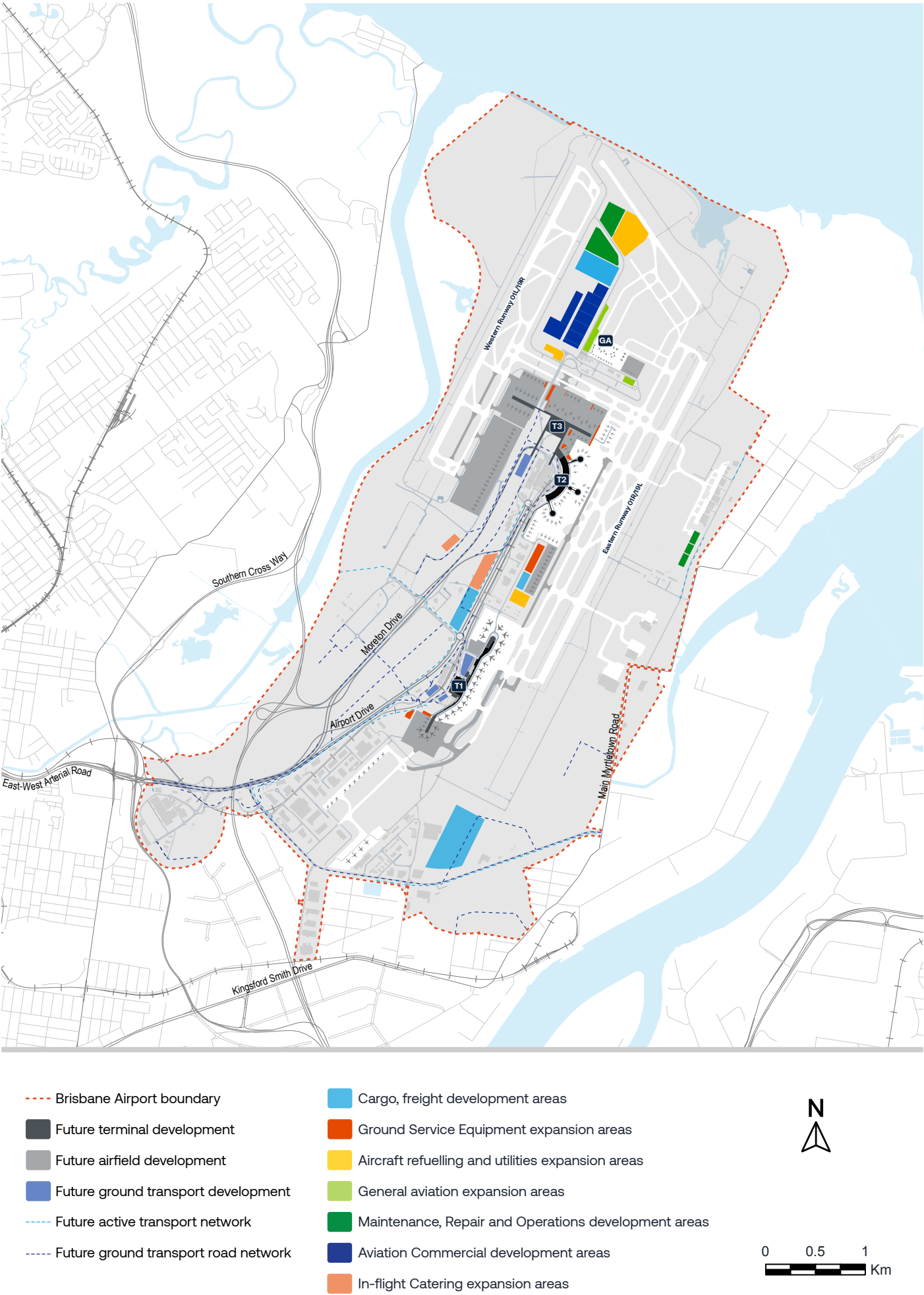
FIGURE 11.6: AVIATION SUPPORT FACILITIES SAFEGUARDING
