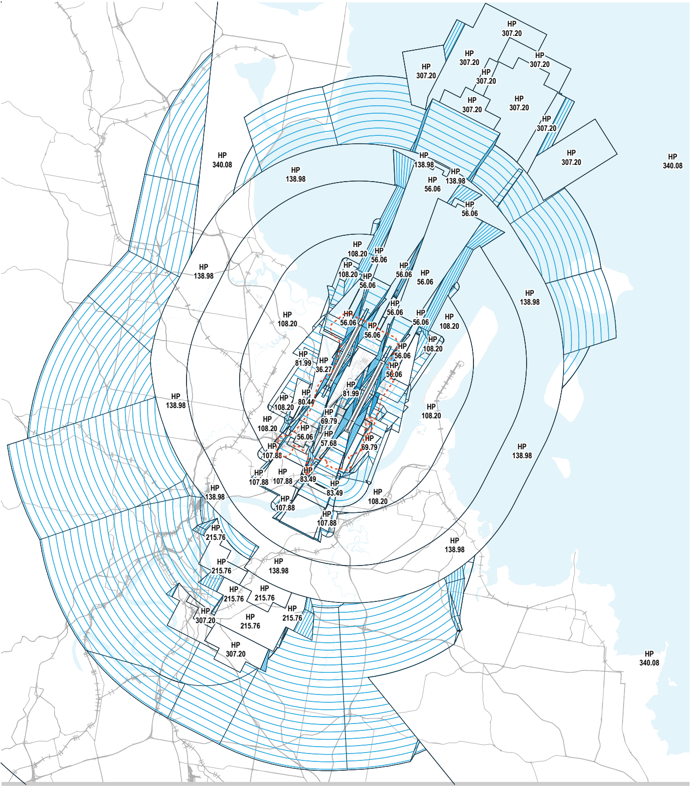
FIGURE 7.5: PROCEDURES FOR AIR NAVIGATION SERVICES – AIRCRAFT OPERATIONS (PANS-OPS)
