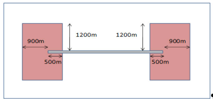
Figure 5: Risk envelope around runways within which buildings should be assessed for windshear and turbulence
